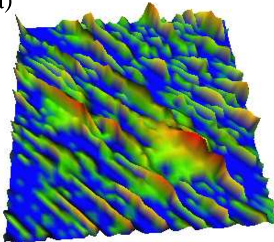
Figure 1: Islands in a local alignment path graph. (a) is a schematic representation of the path graph. In every cell C the red line recalls the choice made by the optimization procedure of the Smith-Waterman algorithm. By these lines, all the cells with non-zero scores are partitioned into islands according to which anchoring points (circles) they are connected to. (b) shows the score landscape on a 50 \times 50 path graph. The score at every cell of the path graph is represented by its height above the surface and color-coded with zero scores corresponding to blue areas and increasingly red colors for higher scores. The example shown is generated with a BLOSUM-62 scoring matrix, and a score -(11 + k) for each gap of length k . The islands are easily seen.
