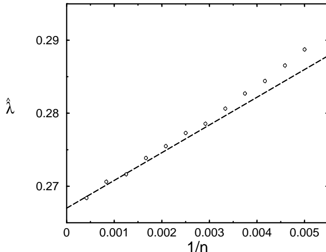
Figure 4: Estimates \hat{\lambda} derived from borderless n \times n sequence comparisons by the island method as a function of 1/n . Approximately 1,000,000 islands with score at least 37 were generated to produce the estimates, which thus have a standard error of 0.1%; the size of the symbols represents one standard error. The plotted line represents the theory of equation [9] for the apparent \tilde{\lambda}(n, n) . The scoring system and random sequence model are the same as those described in the legend to Table 1.
